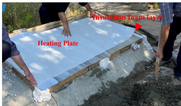
Fig 1 Installation of heating plates on the platform
