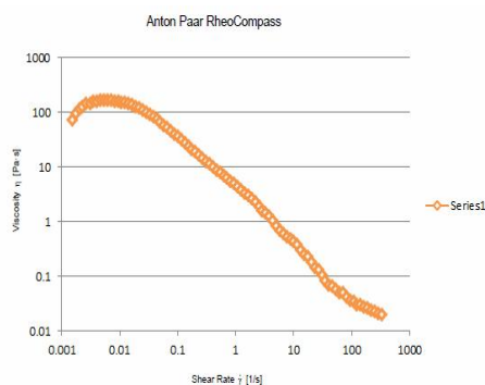
Chart 4 The result of the flow behavior test in sample 3
