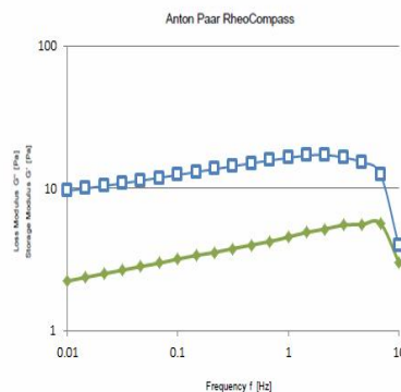
Chart 11 The result of Frequency sweep test in sample 4
