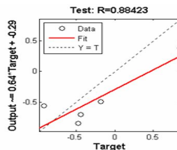
Fig 6 Regression diagram of predicted and actual pH values, a) using 165 Features and b) using 20 Features
