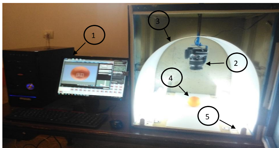
Fig 2 Imaging Set-up: 1- Computer 2- Camera 3- Arched Sheet 4- Sample 5- Monochrome fluorescent lamp (white moonlight)
