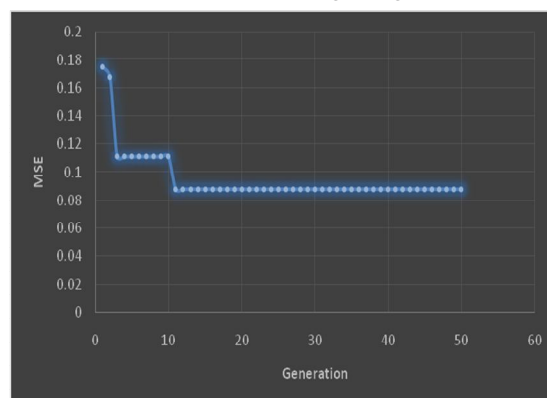
Fig 4 Best fit (least error) versus generation in the artificial neural network optimization process - Genetic algorithm
