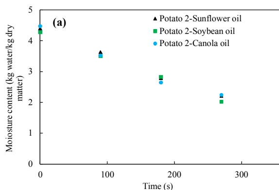
Fig 4 Change in moisture content of potatoes in different oils (a) and in four positions for soybean oil (b)
