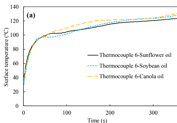
Fig 2 Surface temperature changes (T6) for sunflower, soybean and canola oils (a) and surface temperature changes of four positions fried at soybean oil (b) for the ratio of 1:15
