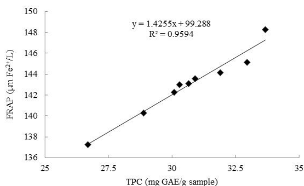
Fig 3 Relationship between total phenolic content, DPPH radical scavenging activity and FRAP for aerial parts of marigold extract.
