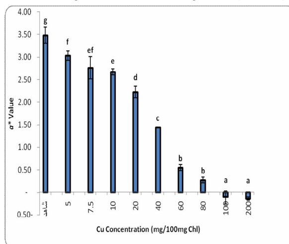
Fig 3 The effect of Cu concentration on the greenness value ( a^* ) of the chlorophyll solution
