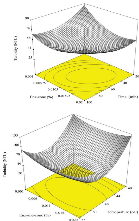
Fig 2 The effect of (a) pectinase concentrations and time (at T = 47.5^{\circ}\text{C} ), and (b) pectinase concentrations and temperature (at t = 60\text{ min} ) on the turbidity.
