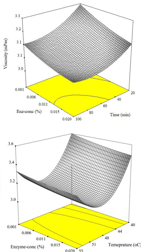
Fig 1 The effect of (a) pectinase concentrations and reaction (at T = 47.5^{\circ}\text{C} ), and (b) pectinase concentrations and temperature (at t = 60\text{ min} ) on the viscosity.
