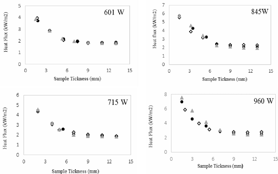
Fig 4 Heat flux changes with respect to sample thickness of Carum carvi seeds with water activity values 0.24 (◇), 0.56 (●) and 0.89 (Δ) at different IR powers.
