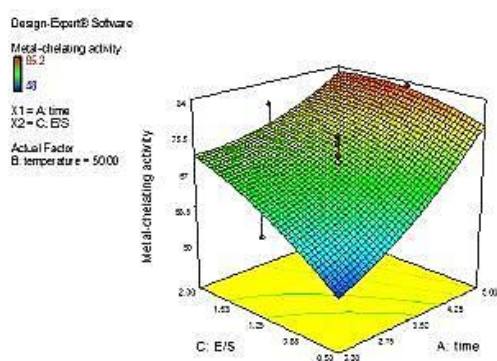
Fig 11 The response surface curve for evaluating the effect of independent variables (Enzyme/Substrate and time) on chelating activity
