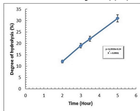
Fig 13 The progress of hydrolysis in the presence of Alkalase
