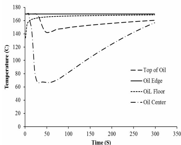
Fig 5 Predicted temperatures for oil during heating at 170°C.
