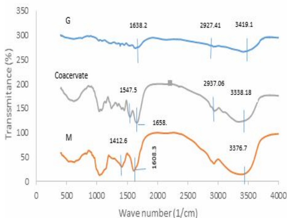
Fig 2 Fourier infrared spectroscopy of gelatin (G), flaxseed mucilage (M) and the coacervate powders
