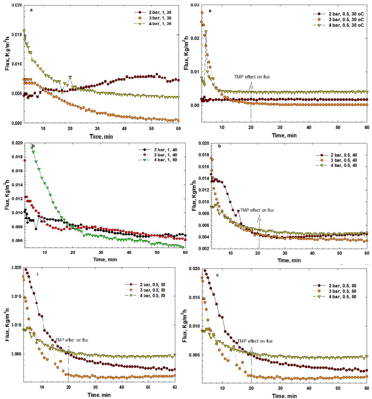
Figure 4 the effect of pressure and flow rate on neutralization of canola oil micella (20:80) at 30 °C (a), 40 °C (b) and 50 °C
