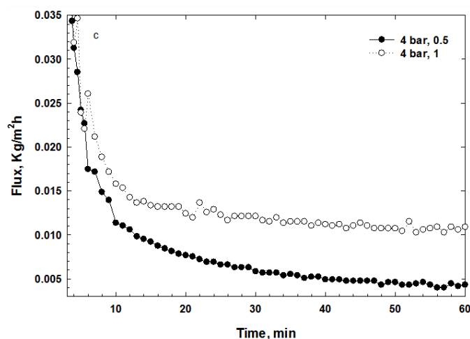
Figure 7 the effect of flow rate on permeate flux through degumming of canola oil micella (30:70)
