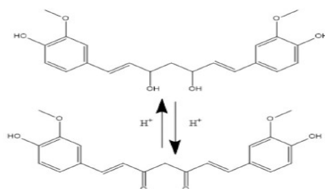
Fig 3 Structural changes of curcumin toward pH changes
