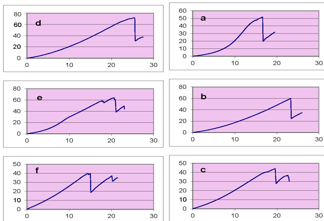
Fig 2 Experimental curves of force-displacement (X-axis: displacement (mm) and Y-axis: force (N)); a, b and c for the samples with m≤500g and loading speed at three levels, 4.5, 7.5 and 10.5 mm/min, respectively) and d, e and f for the samples with m>500g and loading speed at the same levels, respectively)
