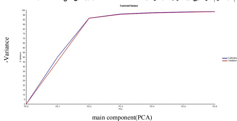
Fig 3 Described variances and factors used in PCA method in the classification of research treatments
