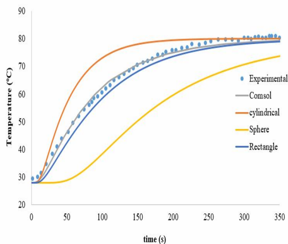
Fig 5 Comparison of temperature determined by experimentation and prediction using analytical and numerical models at 80 °C
