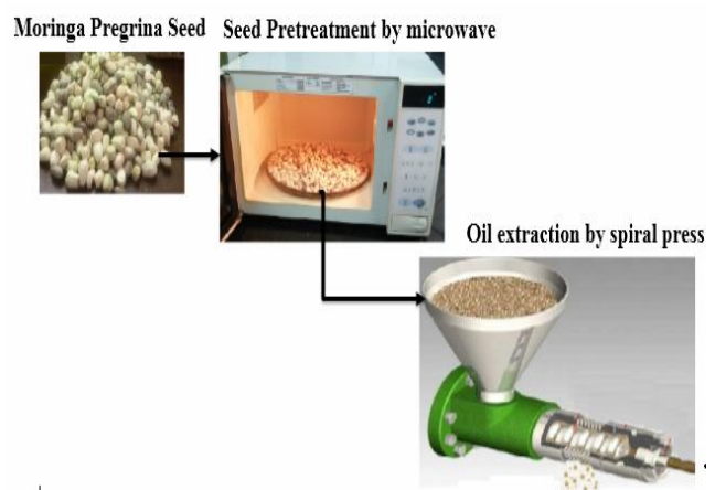
Fig 2 Schematic of mechanical extraction of oil from Moringa seeds.
