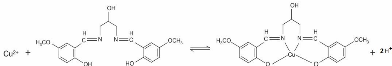
Fig 3 The complexation reaction between Cu(II) and N,N'-bis(5-methoxy-salicylidene)-2-hydroxy-1,3-propanediamine [28]
