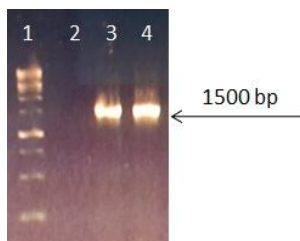
Fig 1 Gel electrophoresis of the PCR products. Lane 1: DNA ladder, lane 2: negative control, lane 3: positive control and lane 4: amplified DNA of the LAB isolate.
