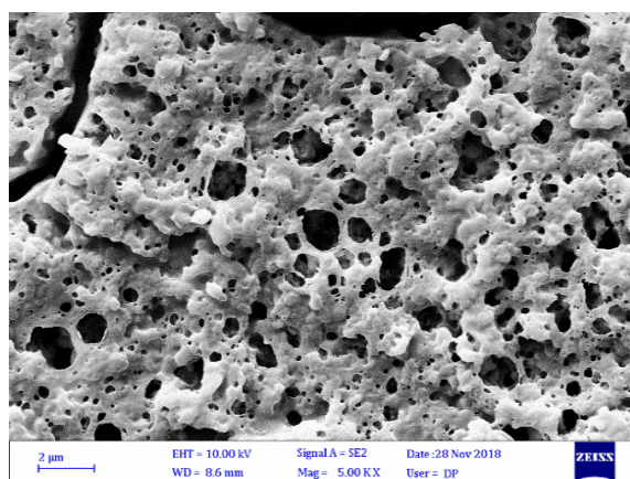
Fig 3 SEM for sodium caseinate / \beta -cyclodextrin microcapsules with cinnamon essential oil.
