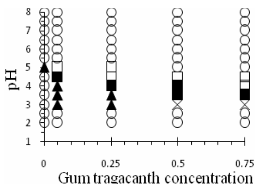
Fig 1 State diagram of aqueous solution system in a wide range of pH (2-8) as a function of gum concentration. The amount of protein in the entire samples is 0.5% (w/w). The solubility/insolubility was evaluated by visual observation: (O) clear solution, (□) cloudy/milky solution, (■) precipitation and cloudy solution, and (▲) precipitation and clear solution.
