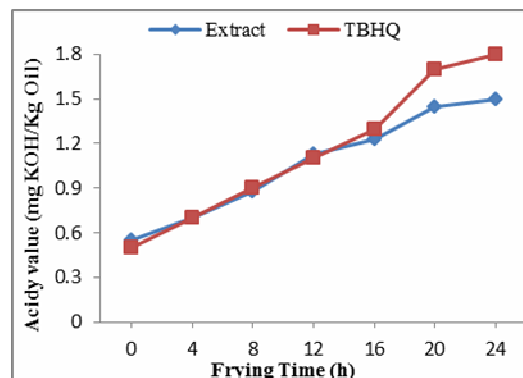
Fig 7 Change in acidity value of sunflower oil during frying at 180°C
