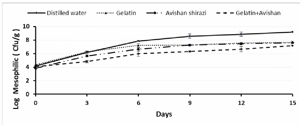
Fig 1 Mean Changes of logarithm of mesophilic bacteria of ostrich fillet during 15 days of storage in refrigerator temperature.
