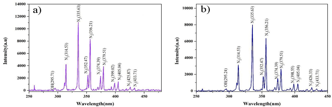
Fig 4 Optical emission spectrum of dielectric barrier discharge plasma in a) surface mode b) volumetric mode
