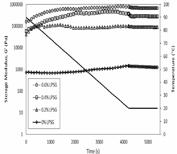
Fig 2 The effect of cooling process from 90 to 20°C on the elastic modulus of different ratios of LSPI-LPSG mixed gel (rate of 1 °C/min and holding for 20 minutes, 1 Hz, strain 0.5%).
