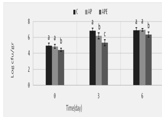
Fig 3 Effect of treatments on E.coli O157:H7 during 6 days of storage at 4 \pm 1^{\circ}\text{C} (C:control+ E.coli , AP:control+ E.coli + acidophilus + plantarum , APE:control+ E.coli + acidophilus + plantarum +EDTA)
