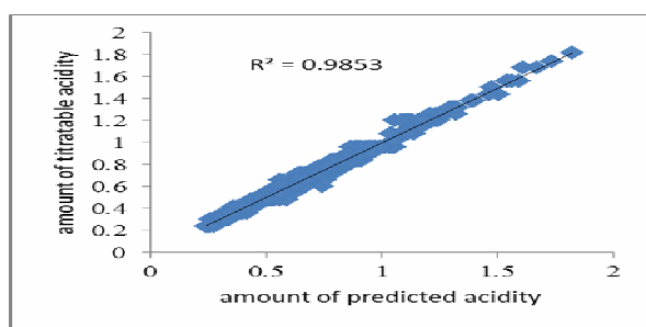
Fig 2 The variation of predicted acidity versus titratable acidity: a) Newcf network with hyperbolic sigmoidal tangent activation function, b) Newcf network with hyperbolic sigmoidal logarithm activation function, c) Newff network with hyperbolic sigmoidal tangent activation function, d) Newff network with hyperbolic sigmoidal logarithm activation function
