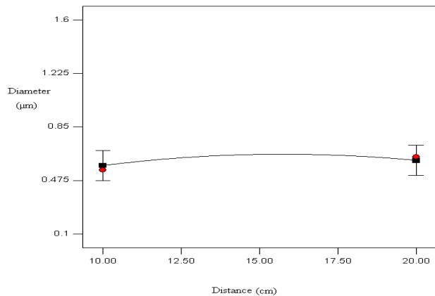
Figure 5 Influence of Distance between needle tip and collector (cm) on fiber diameter ( \mu\text{m} ) in electrospinning at a constant zein solution concentration of 26 w/v %, voltage of 20 kV and flow rate of 8 ml/h.
