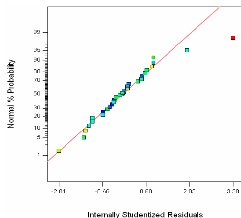
Figure 6 The probability of normality for residuals
