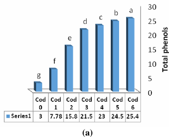
Fig 1 The results of total phenol for different treatments of ice cream (mg/µg), b) standard curve by Folin-Ciocalteu absorption of gallic acid
