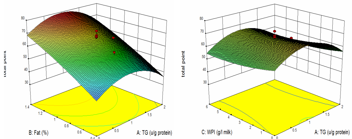
Fig 7 Response surface plots for interaction effects of formulation ingredients on total sensory score of low-fat Iranian white cheese incorporated with whey protein isolate and treated with transglutaminase
