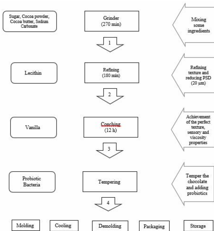
Fig 1 Scheme of Scheme of Probiotic Dark Chocolate (PDC) manufacturing process (adapted from 1).
