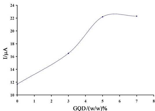
Fig 2 The effect of graphene-quantum dot nanoparticles (w/w %) on current of sunset yellow at the modified sensor
