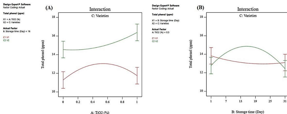
Fig 5 Interaction of TiO_2 and storage time with varieties ( V_1 ) Hosseini, and ( V_2 ) Ghezal Ozom on total phenol
