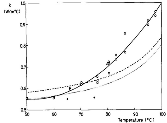
Fig4 Potato heat transfer coefficient [2].
