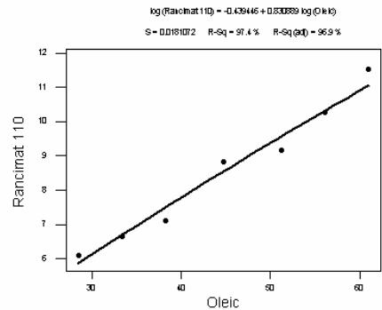
regression between % oleic and stability
