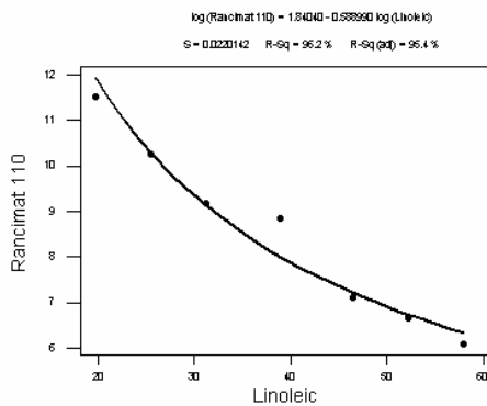
regression between % Linoleic and stability
