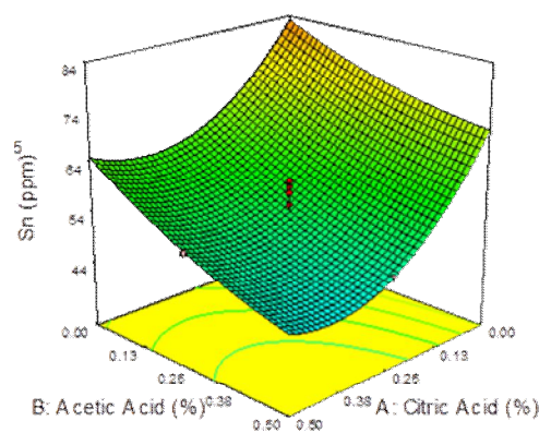
Fig 7 The surface contour of Citric Acid and Acetic Acid effects on Tin content during blanching (5minutes)
