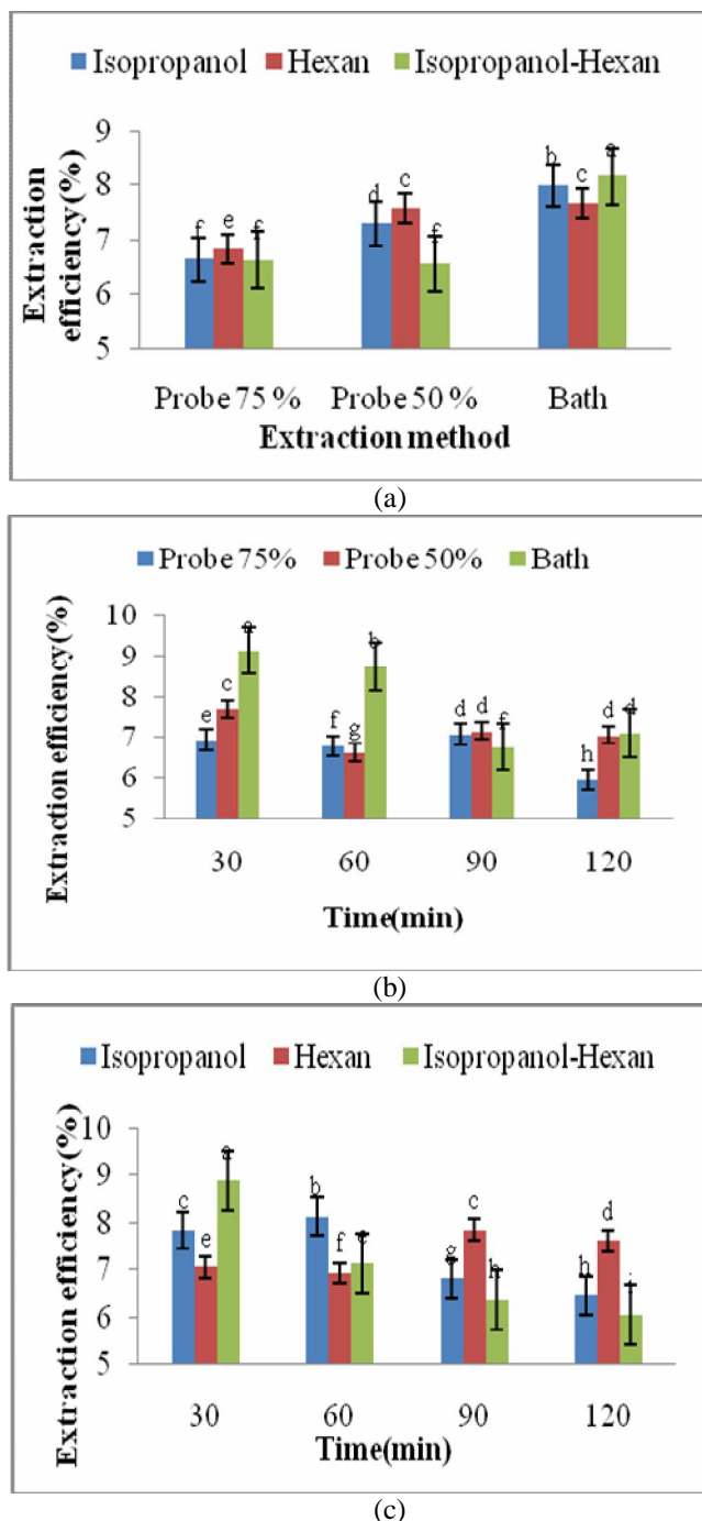
Fig 1 Interaction effect of type of extraction method \times solvent (a), extraction method \times time (b), time \times solvent on extraction efficiency. Different letters indicated significant statistical different between soybean oil samples
