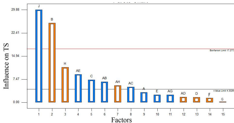
Fig 1 Pareto chart
