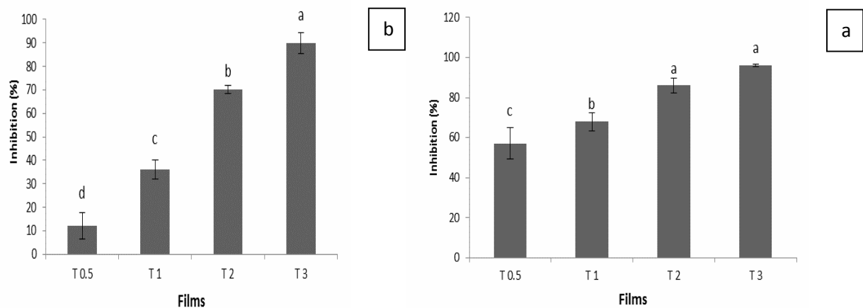
Fig 7 Effect of different amounts of \text{TiO}_2 on antimicrobial activity of bilayer pectin-carnauba film against E. coli at 6 (a) and 24 (b) incubation at 37 °C (T: \text{TiO}_2\% )
