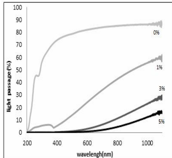
Fig 2 The effect of zinc oxide on the light passage of Qodume Shirazi gum films at wavelengths of 200-1100 nm.
