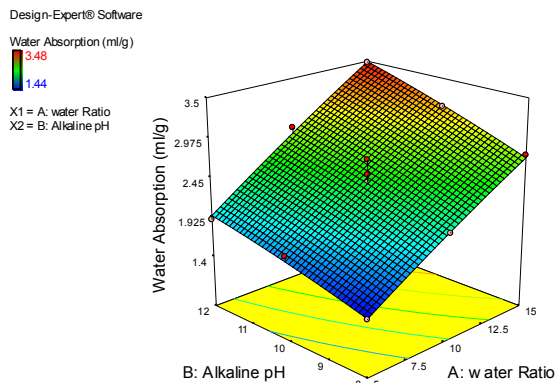
Fig 5 Effect of alkaline pH and water ratio on water absorption
